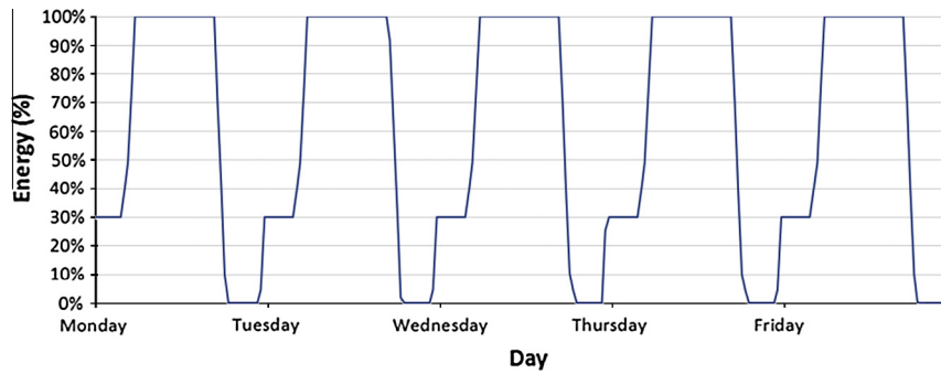
Fig. 11. Storage scheduled state of charge over a week for longer-term commitments.
