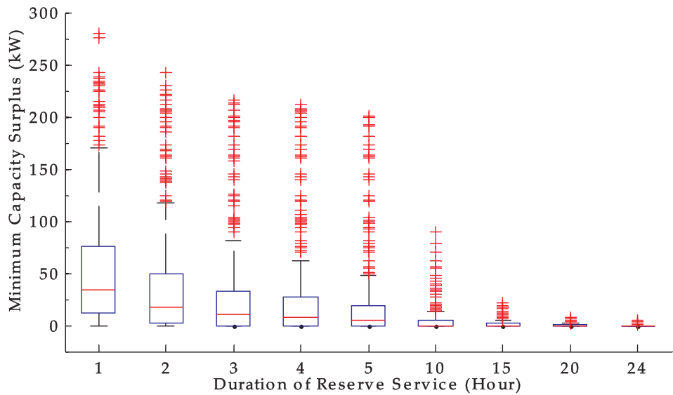
Fig. 8. Probabilistic capacity tables of MG2 presented as boxplots with consideration of various durations of reserve service.
