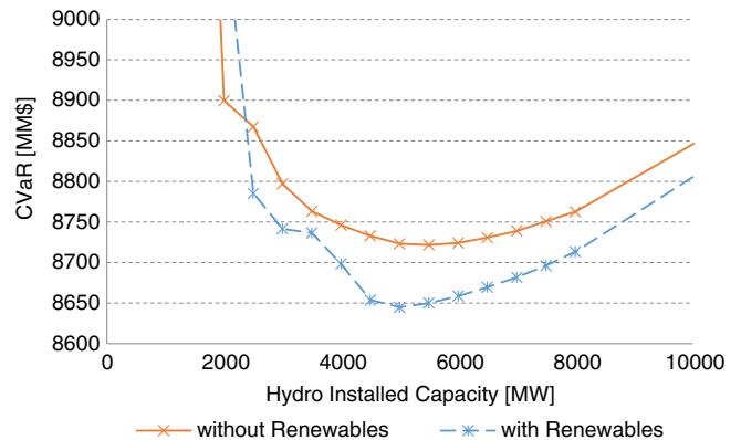
Fig. 5. CVaR versus hydro (reservoir) installed capacity with and without renewables.
