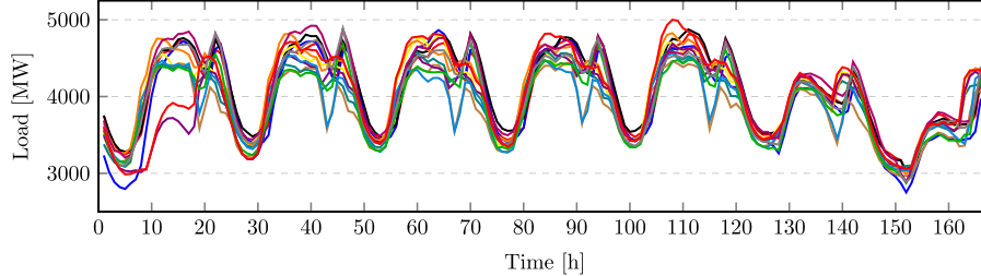
(a) Representative load profiles
