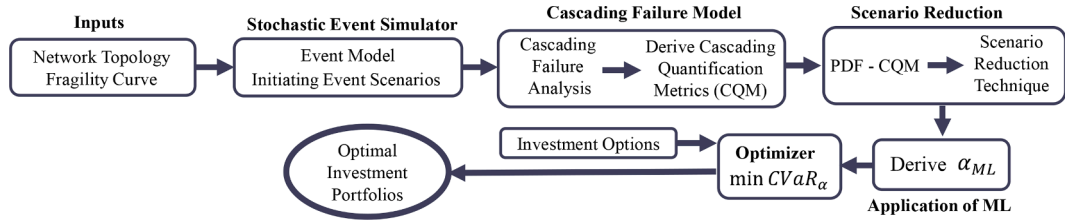
Fig. 1. Overview of the proposed framework.
