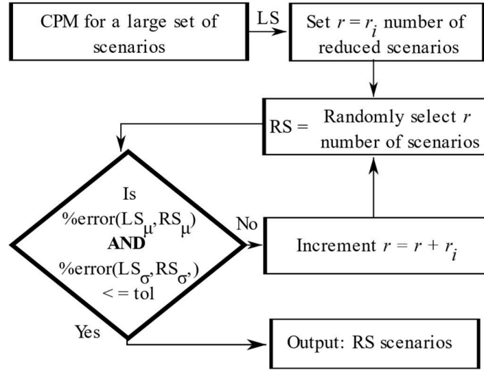
Fig. 2. Flowchart of proposed scenario reduction technique.
