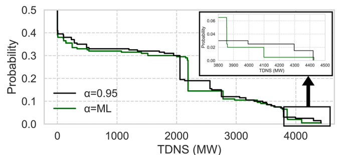
Fig. 4. Comparison of CCDF of TDNS between proposed approach with \alpha = 0.95 and \alpha_{ML} .
