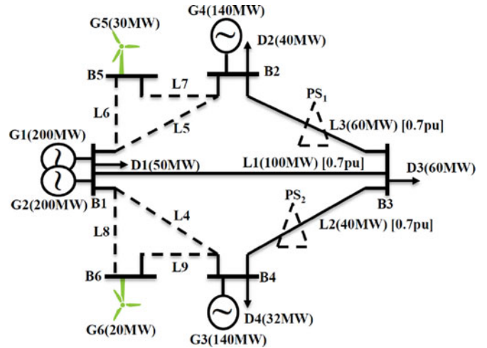
Fig. 4. Generation, network, and demand data of 6-Bus system, where continuous lines refer to existing infrastructure and dashed lines refer to candidate infrastructure. Normal brackets refer to generation and network capacities and peak demand conditions, while square brackets refer to reactances.
