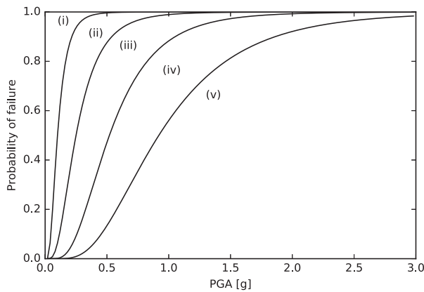
Fig. 3. Generator's fragility curves with five states. (i) No damage. (ii) Minor. (iii) Moderate. (iv) Extensive. (v) Complete damage.
